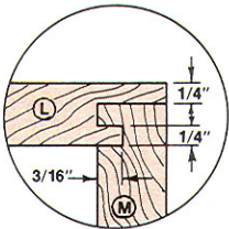
DRAWER JOINT DETAIL
