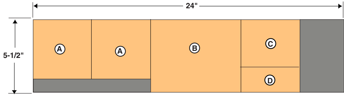
CUTTING DIAGRAM FOR WREN HOUSE
