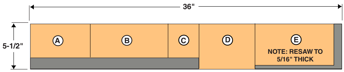
CUTTING DIAGRAM FOR BLUE JAY HOUSE
