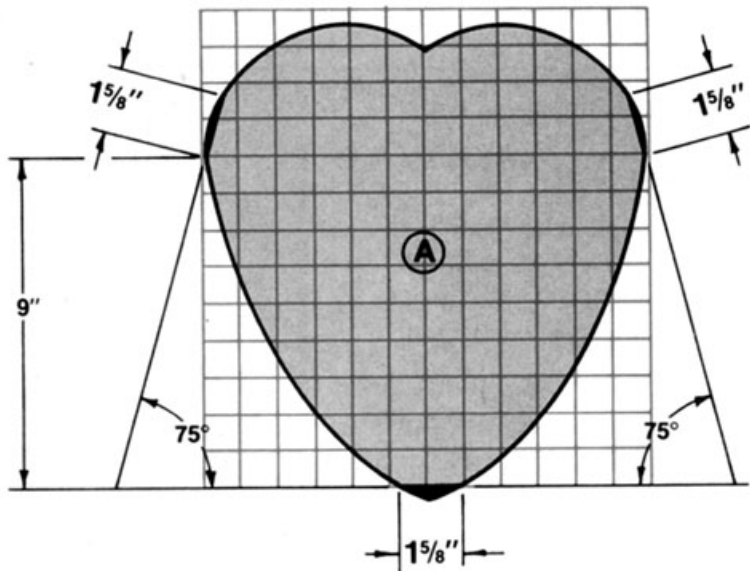
FIGURE 2 SHELF DESIGN
