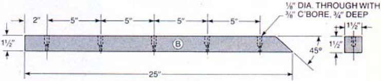
LEG BRACE (4) REQ'D.
