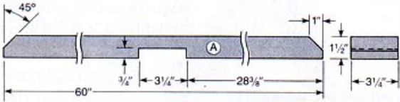
FOOT INNER LEG SET (1) REQ'D.
