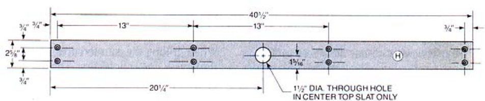
TOP SLAT (15) REQ'D.
