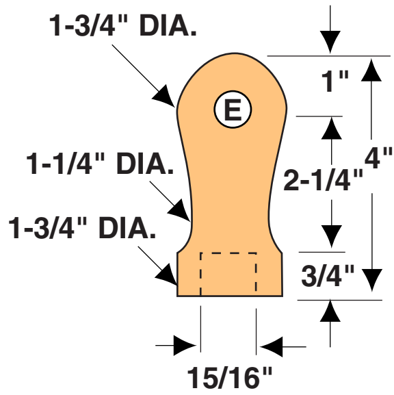
HANDLE DETAIL
