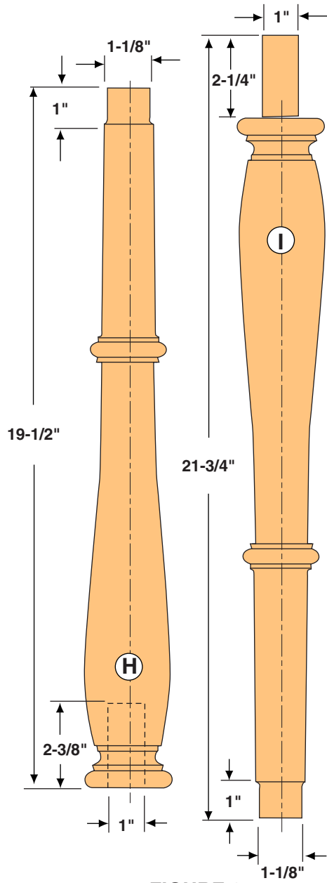
FIGURE 6 BLANKET RAIL SPINDLES
