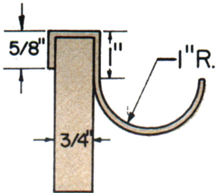
HOOK DETAIL
