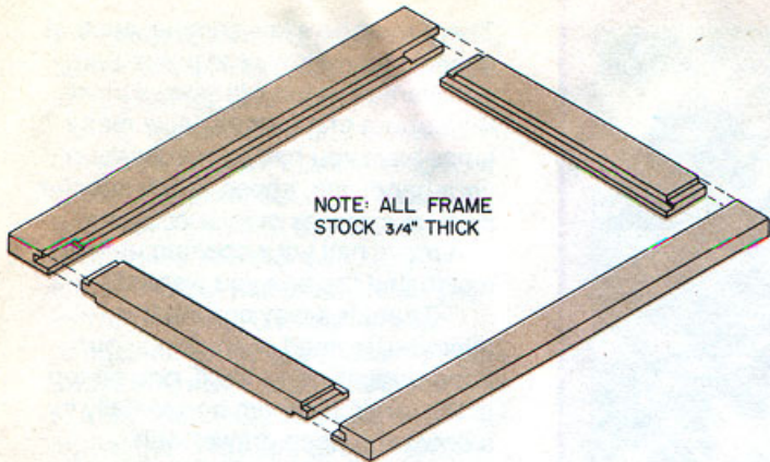
CABINET DOOR FRAME ASSEMBLY
